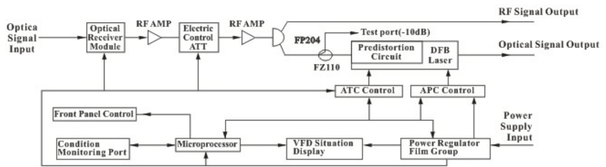
1310nm Indoor Laser Transmitter Block Diagram
