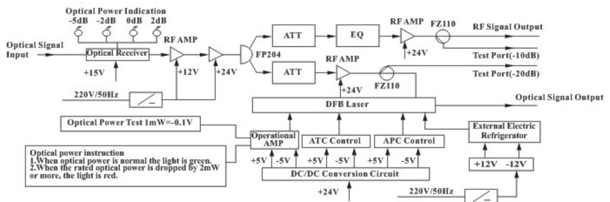
1310nm Outdoor Laser Transmitter Block Diagram
